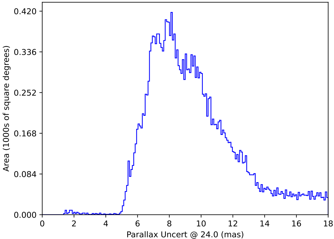
roll_pause_mjdp270_v3.4_10yrs All sky: Parallax Uncert @ 24.0
