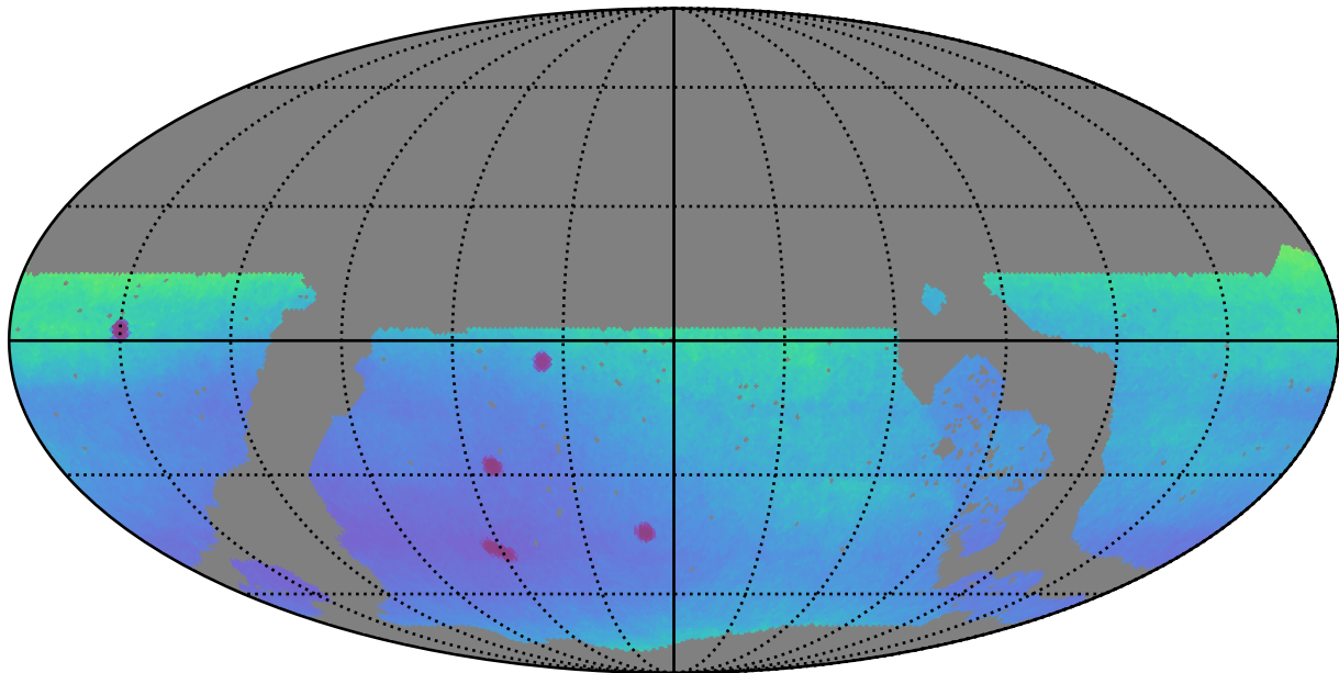
roll_pause_mjdp270_v3.4_10yrs WFD: Parallax Uncert @ 22.4
