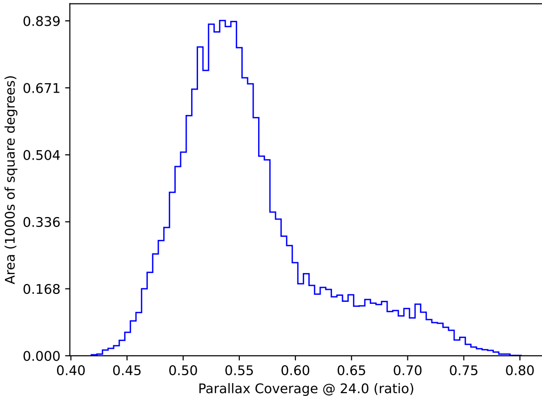
roll_pause_mjdp270_v3.4_10yrs WFD: Parallax Coverage @ 24.0
