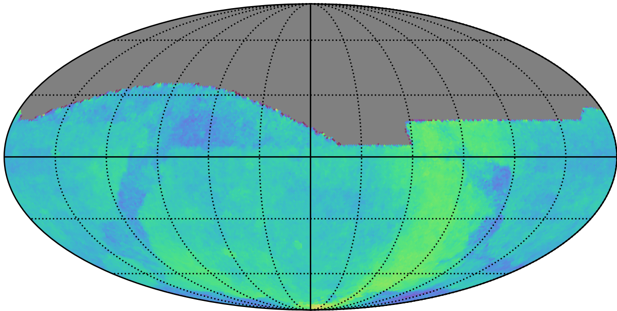
roll_pause_mjdp270_v3.4_10yrs All sky: Parallax Coverage @ 24.0
