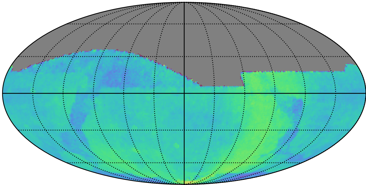
roll_pause_mjdp270_v3.4_10yrs All sky: Parallax Coverage @ 22.4
