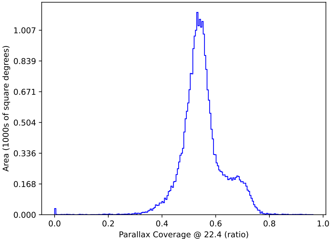
roll_pause_mjdp270_v3.4_10yrs All sky: Parallax Coverage @ 22.4
