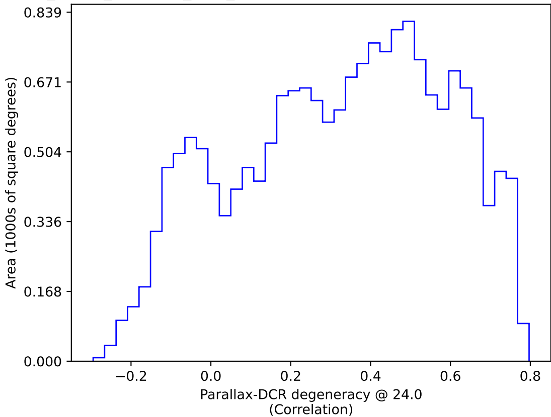
roll_pause_mjdp270_v3.4_10yrs WFD: Parallax-DCR degeneracy @ 24.0
