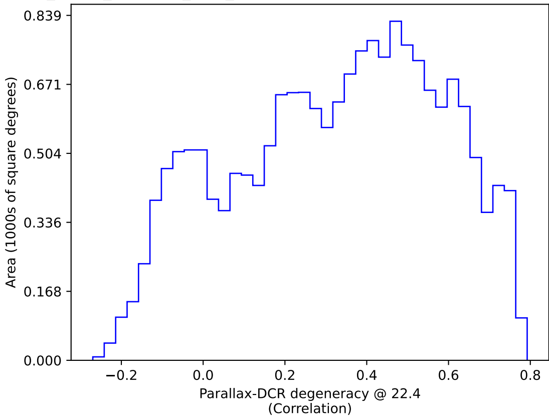
roll_pause_mjdp270_v3.4_10yrs WFD: Parallax-DCR degeneracy @ 22.4
