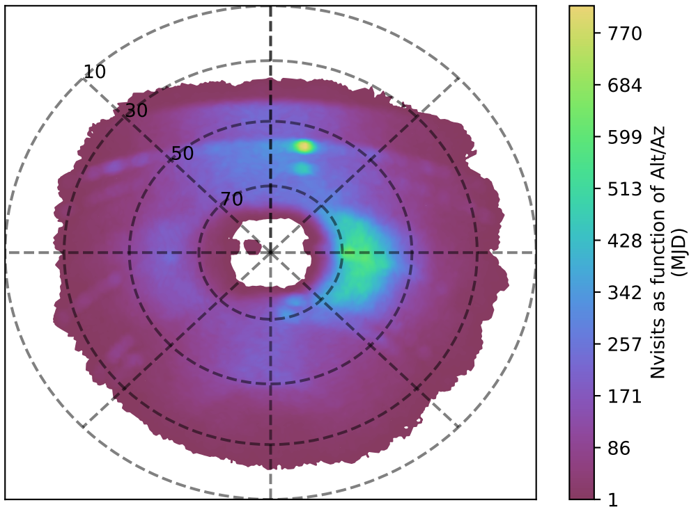
roll_pause_mjdp270_v3.4_10yrs u band: Nvisits as function of Alt/Az
