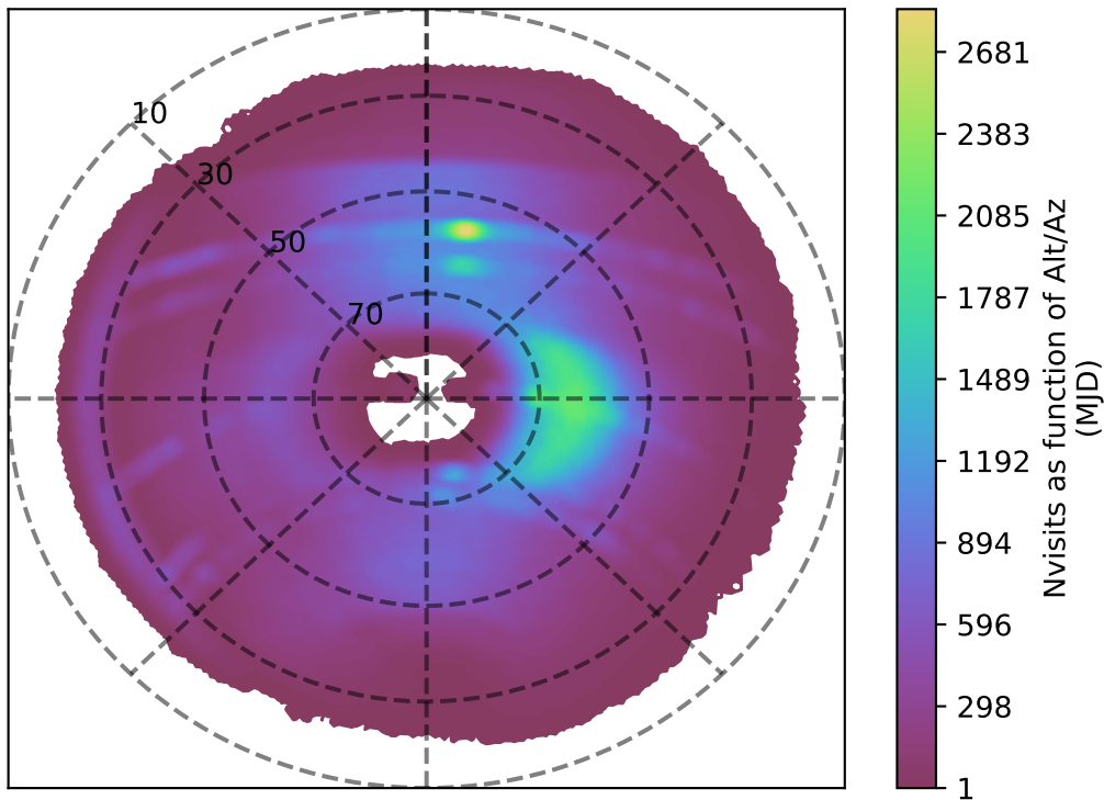
roll_pause_mjdp270_v3.4_10yrs r band: Nvisits as function of Alt/Az
