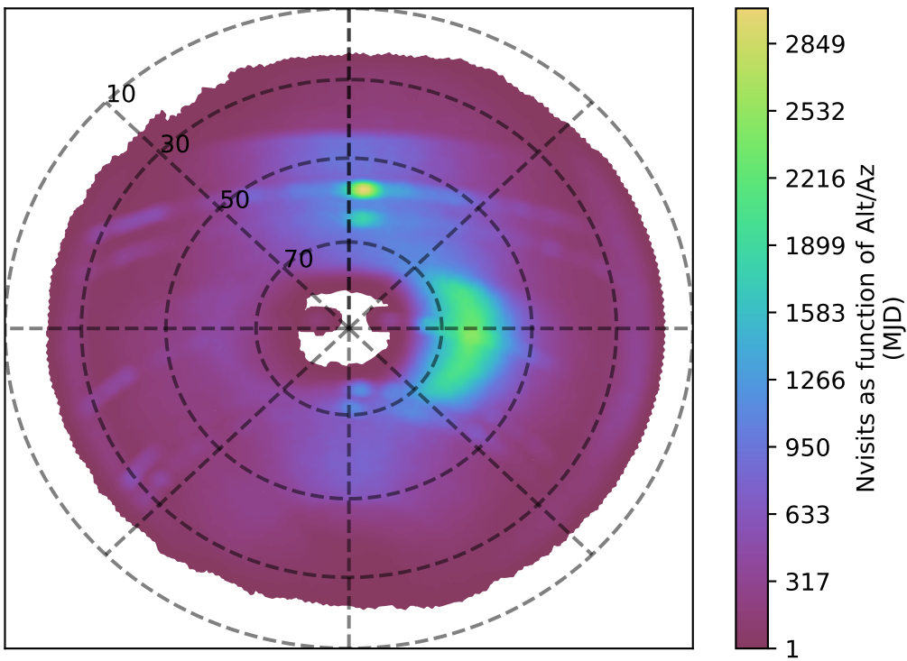
roll_pause_mjdp270_v3.4_10yrs i band: Nvisits as function of Alt/Az
