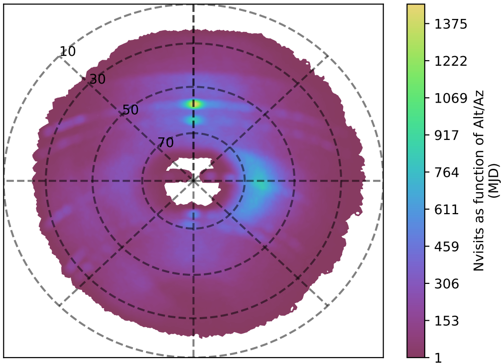
roll_pause_mjdp270_v3.4_10yrs g band: Nvisits as function of Alt/Az
