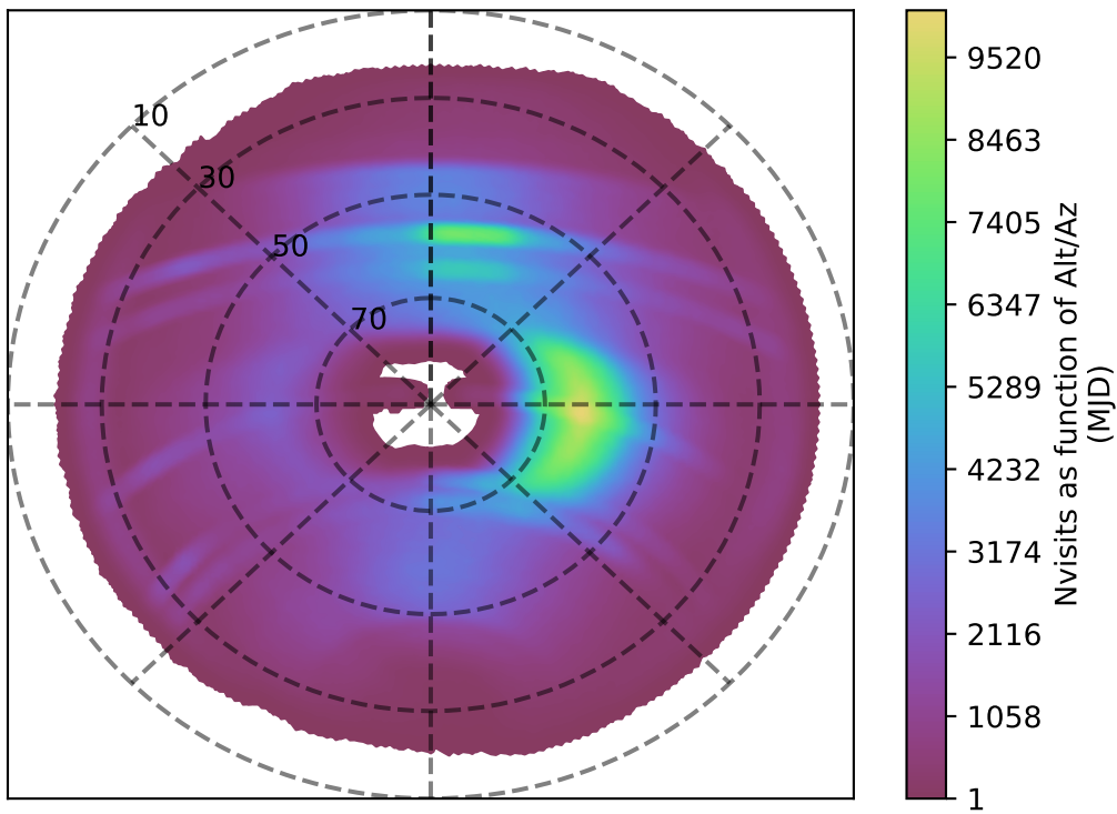
roll_pause_mjdp270_v3.4_10yrs all bands: Nvisits as function of Alt/Az
