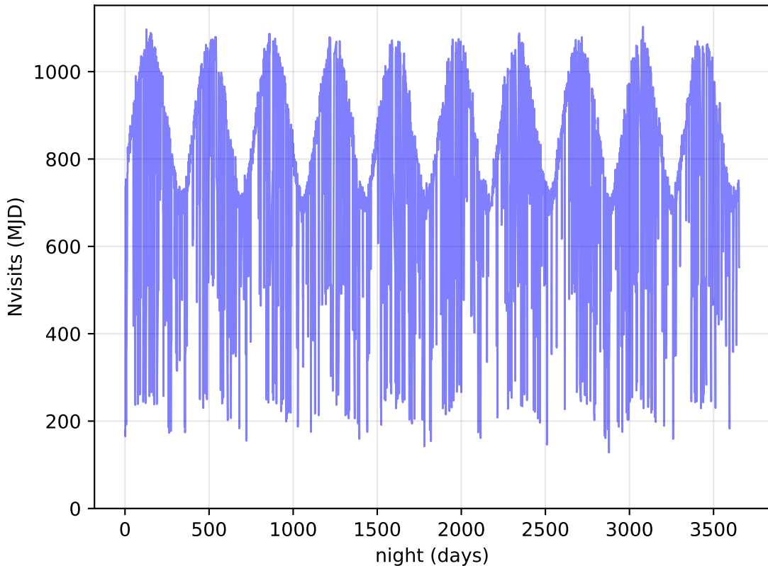
roll_pause_mjdp270_v3.4_10yrs All visits: Nvisits
