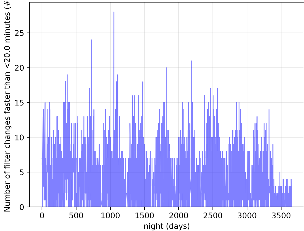
roll_pause_midp270_v3.4_10yrs Per Night: Number of filter changes faster than <20.0 minutes
