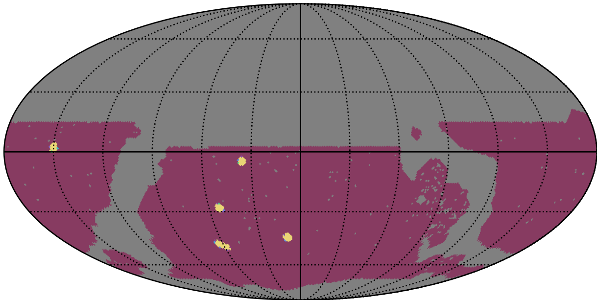
roll_pause_mjdp270_v3.4_10yrs WFD: NumberOfQuickRevisits
