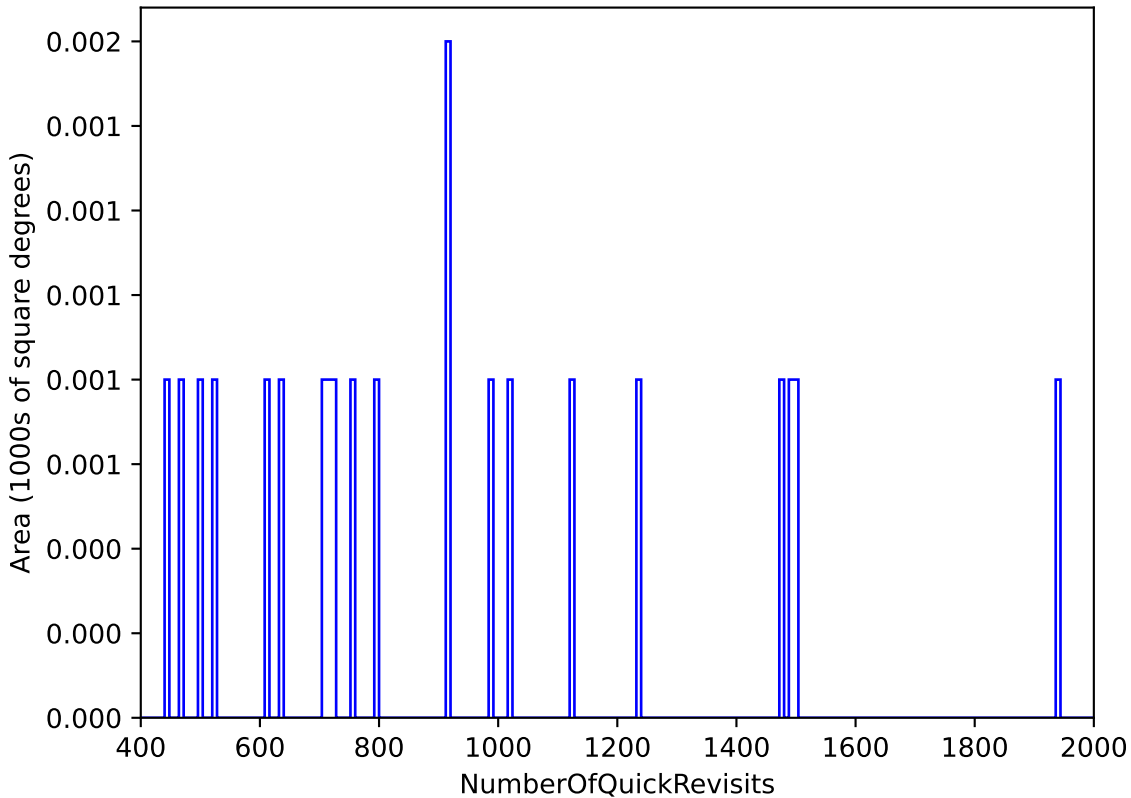
roll_pause_mjdp270_v3.4_10yrs WFD: NumberOfQuickRevisits
