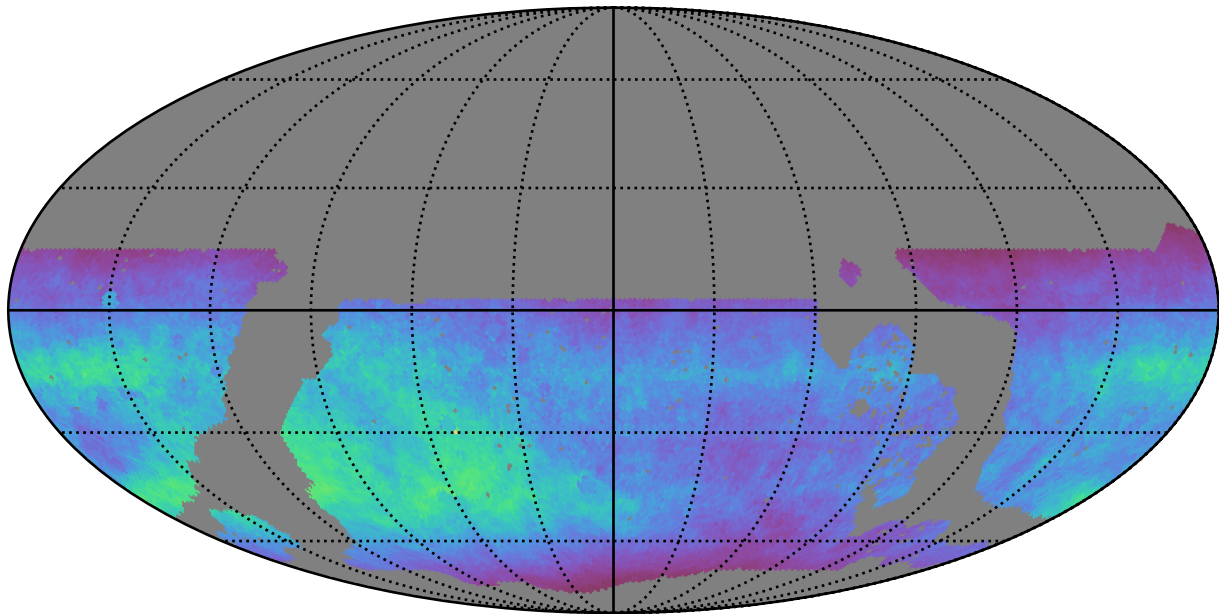
roll_pause_mjdp270_v3.4_10yrs WFD z band: Normalized Teff
