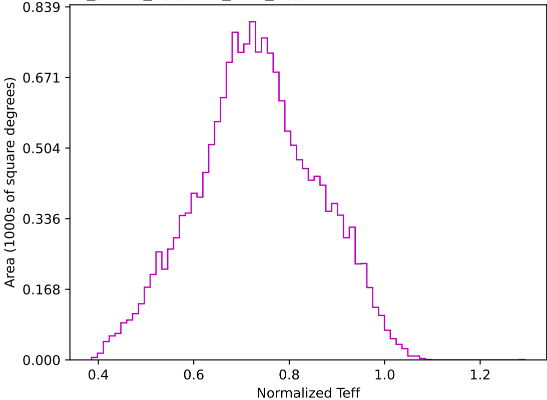
roll_pause_mjdp270_v3.4_10yrs WFD z band: Normalized Teff
