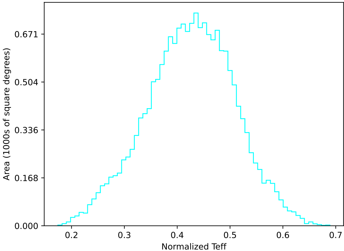
roll_pause_mjdp270_v3.4_10yrs WFD u band: Normalized Teff
