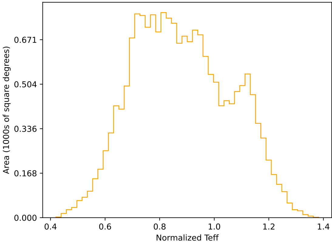
roll_pause_mjdp270_v3.4_10yrs WFD r band: Normalized Teff
