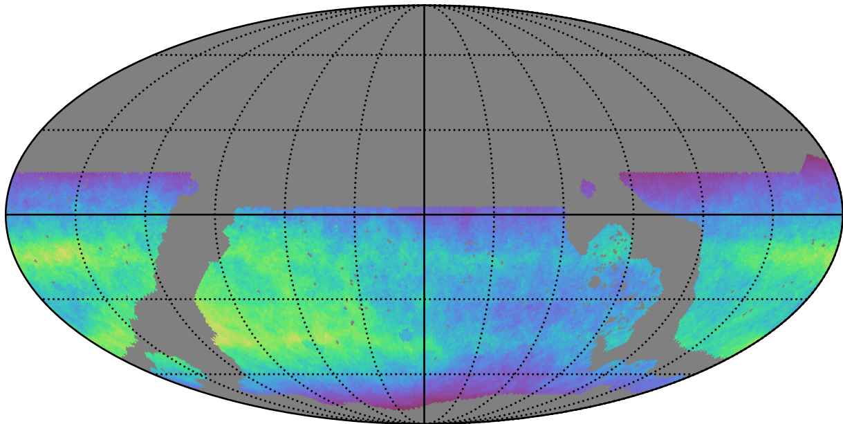
roll_pause_mjdp270_v3.4_10yrs WFD i band: Normalized Teff
