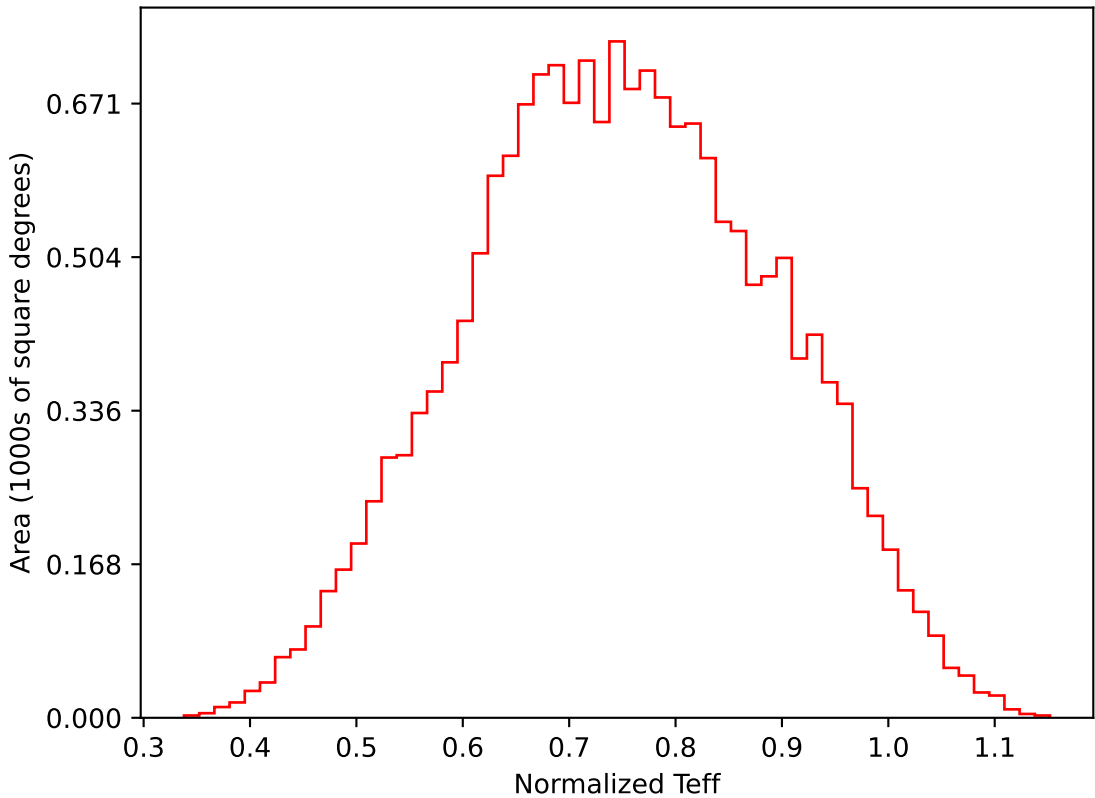
roll_pause_mjdp270_v3.4_10yrs WFD i band: Normalized Teff
