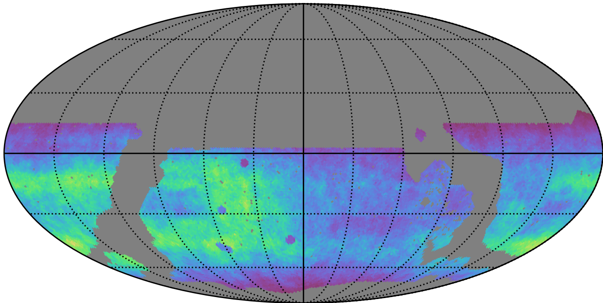
roll_pause_mjdp270_v3.4_10yrs WFD g band: Normalized Teff
