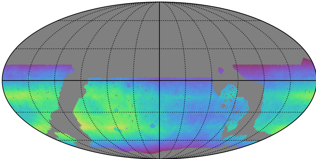
roll_pause_mjdp270_v3.4_10yrs WFD all bands: Normalized Teff
