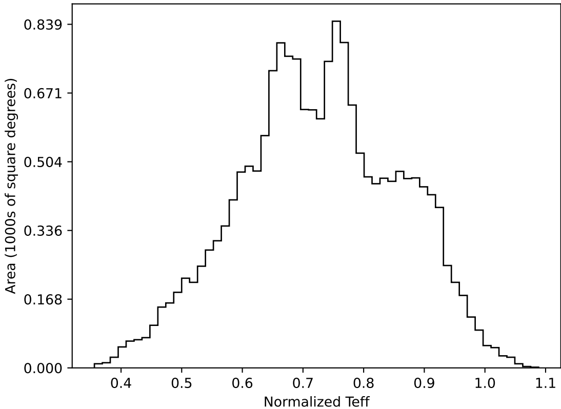
roll_pause_mjdp270_v3.4_10yrs WFD all bands: Normalized Teff
