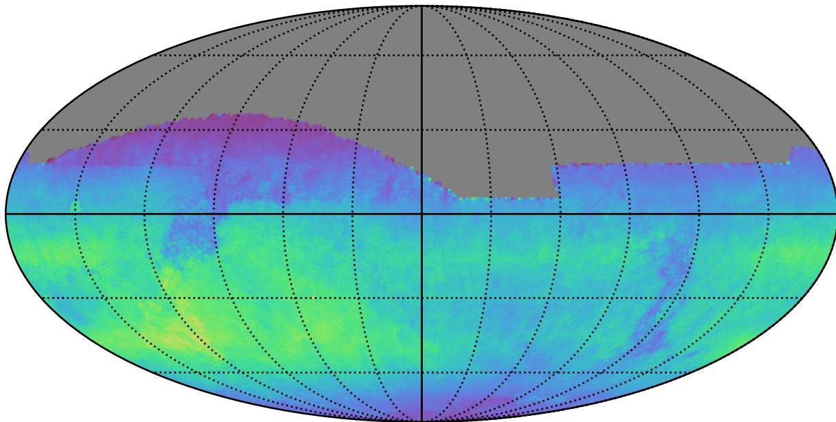
roll_pause_mjdp270_v3.4_10yrs All sky z band: Normalized Teff
