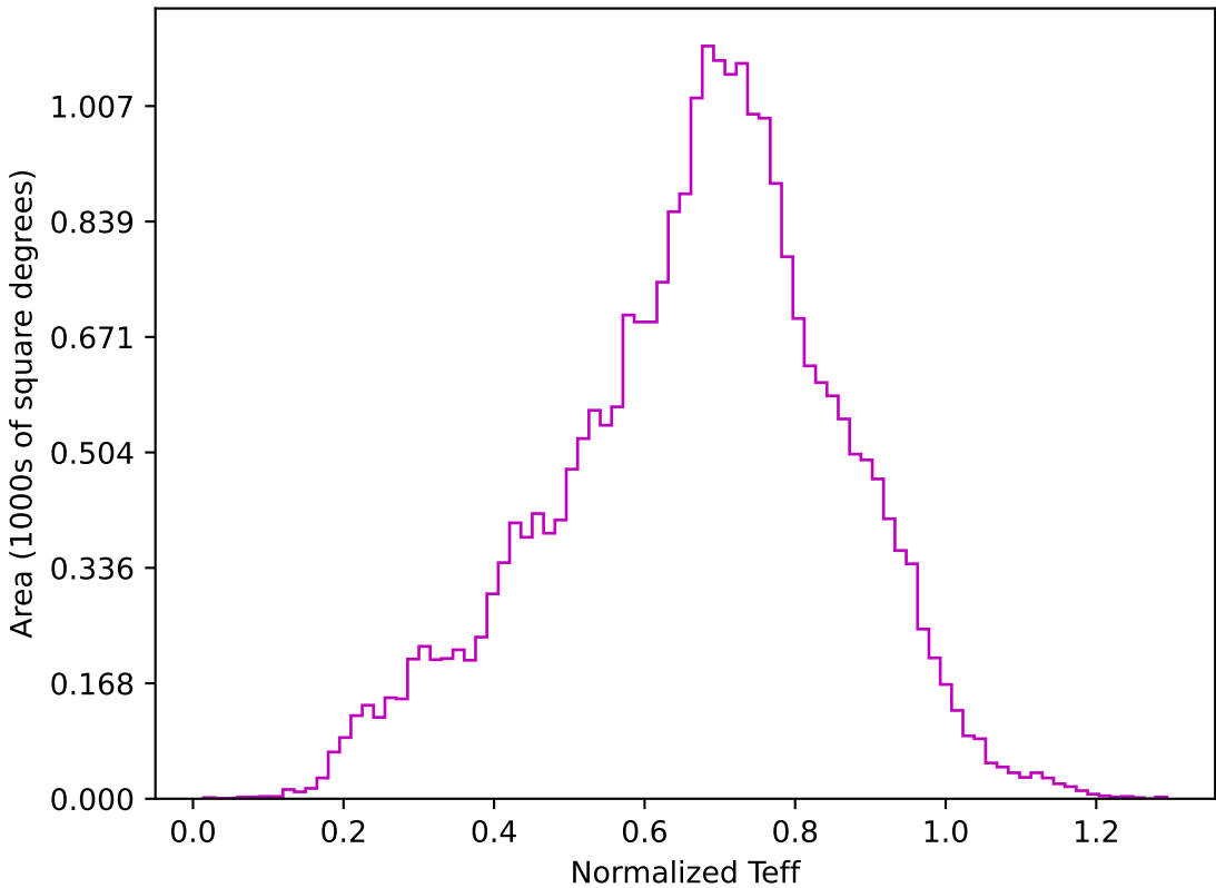
roll_pause_mjdp270_v3.4_10yrs All sky z band: Normalized Teff
