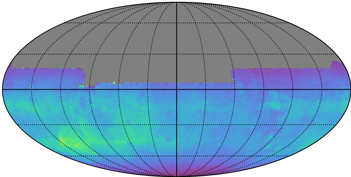
roll_pause_mjdp270_v3.4_10yrs All sky y band: Normalized Teff
