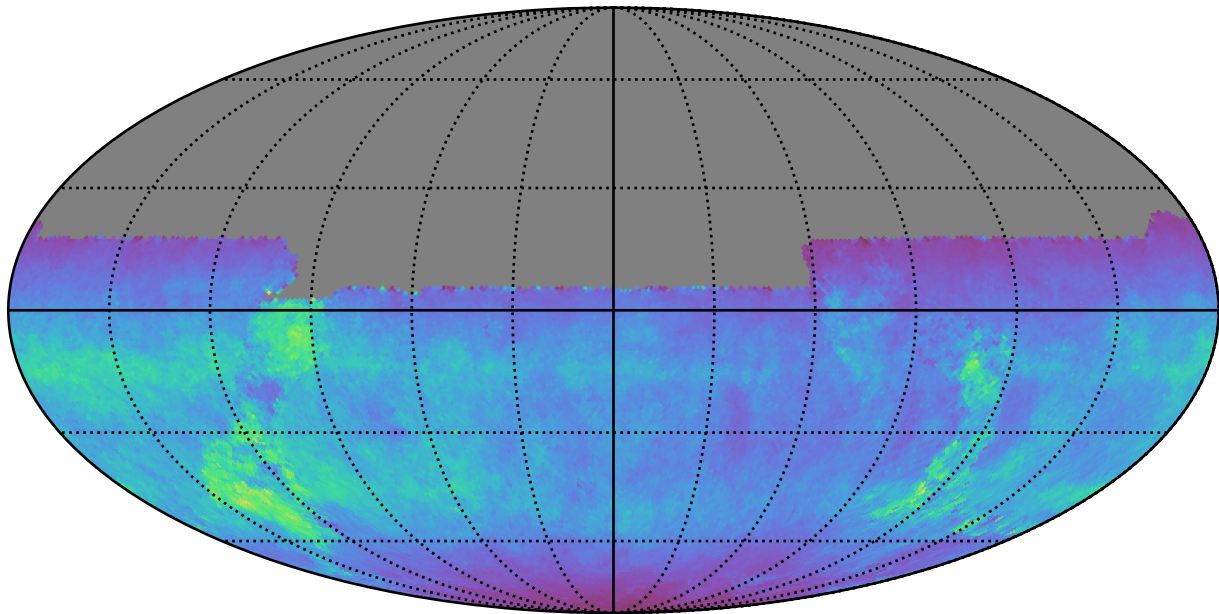
roll_pause_mjdp270_v3.4_10yrs All sky u band: Normalized Teff
