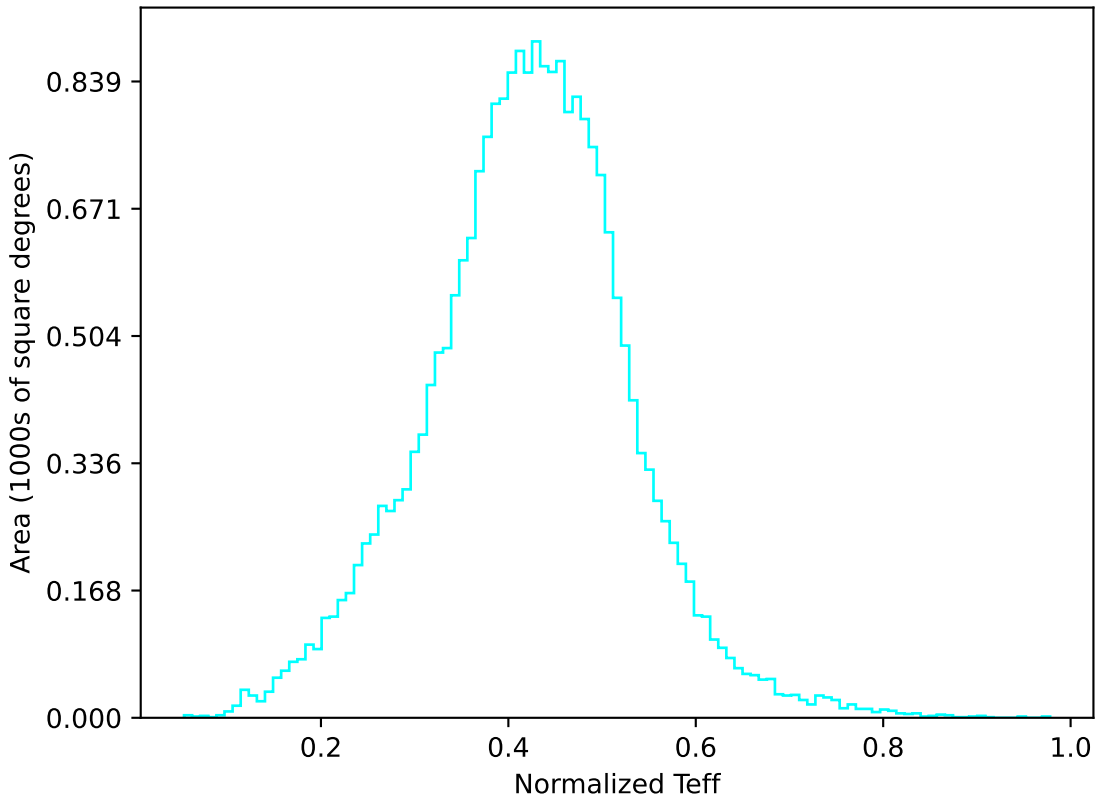
roll_pause_mjdp270_v3.4_10yrs All sky u band: Normalized Teff
