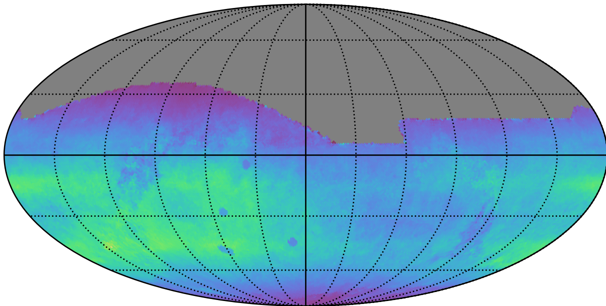
roll_pause_mjdp270_v3.4_10yrs All sky r band: Normalized Teff
