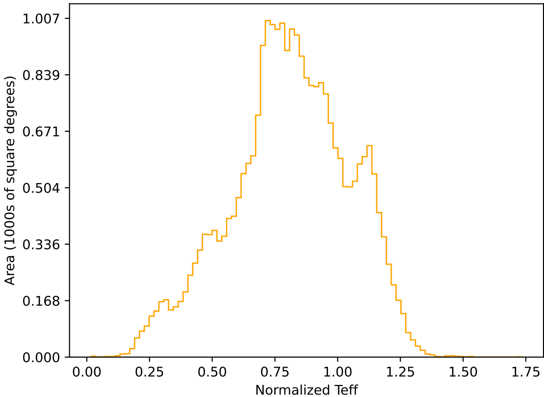
roll_pause_mjdp270_v3.4_10yrs All sky r band: Normalized Teff
