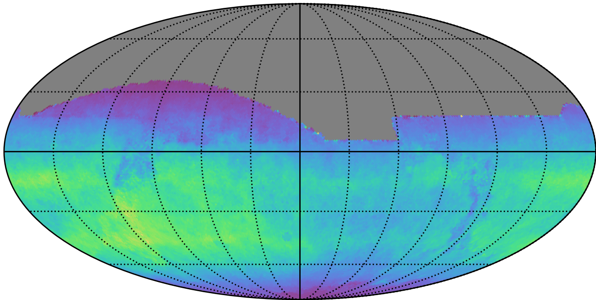
roll_pause_mjdp270_v3.4_10yrs All sky i band: Normalized Teff
