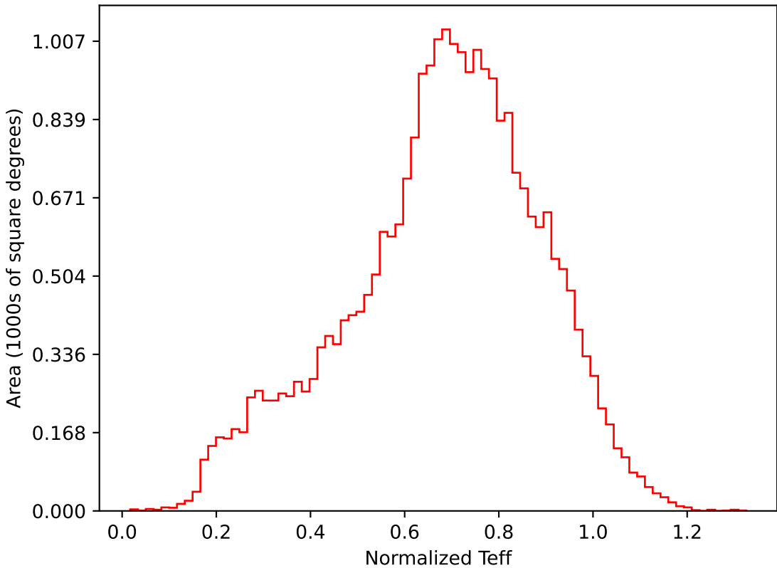
roll_pause_mjdp270_v3.4_10yrs All sky i band: Normalized Teff
