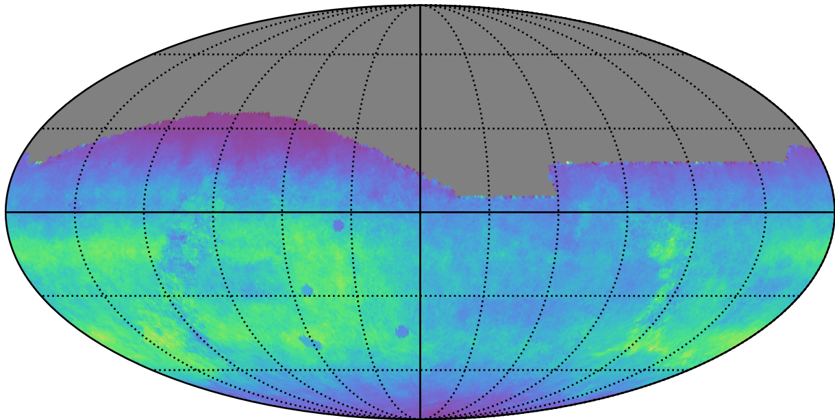
roll_pause_mjdp270_v3.4_10yrs All sky g band: Normalized Teff
