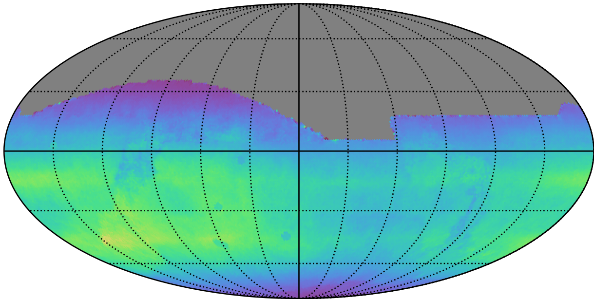
roll_pause_mjdp270_v3.4_10yrs All sky all bands: Normalized Teff
