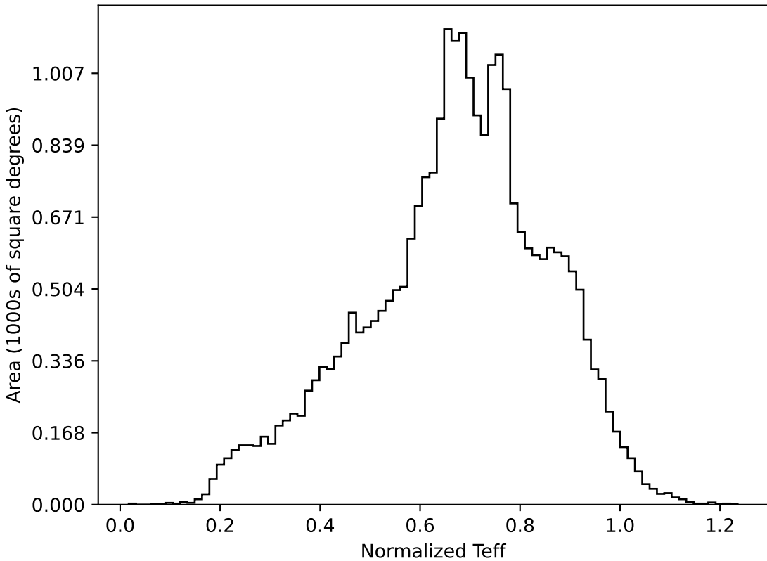
roll_pause_mjdp270_v3.4_10yrs All sky all bands: Normalized Teff
