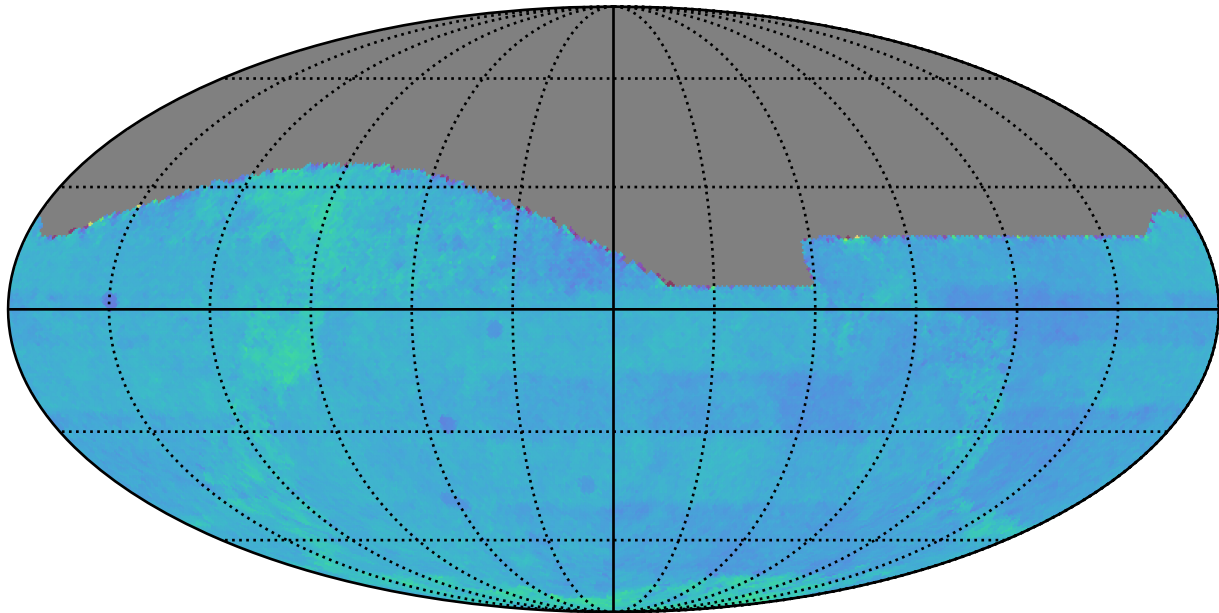
roll_pause_mjdp270_v3.4_10yrs All sky: Normalized Proper Motion Uncert @ 24.0
