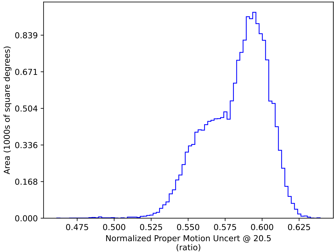
roll_pause_mjdp270_v3.4_10yrs WFD: Normalized Proper Motion Uncert @ 20.5
