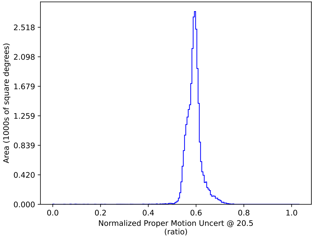
roll_pause_mjdp270_v3.4_10yrs All sky: Normalized Proper Motion Uncert @ 20.5
