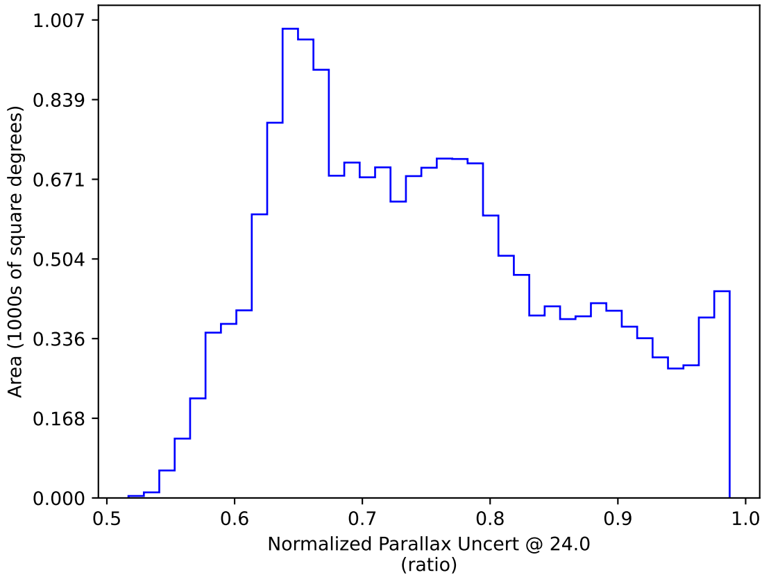
roll_pause_mjdp270_v3.4_10yrs WFD: Normalized Parallax Uncert @ 24.0
