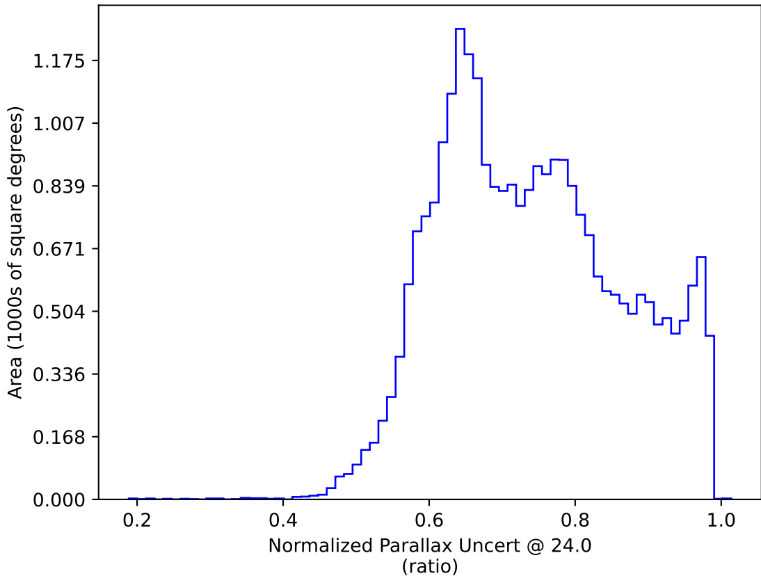
roll_pause_mjdp270_v3.4_10yrs All sky: Normalized Parallax Uncert @ 24.0
