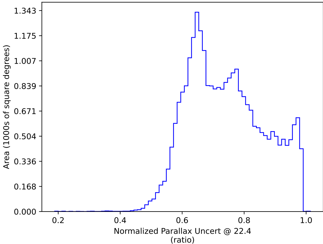
roll_pause_mjdp270_v3.4_10yrs All sky: Normalized Parallax Uncert @ 22.4
