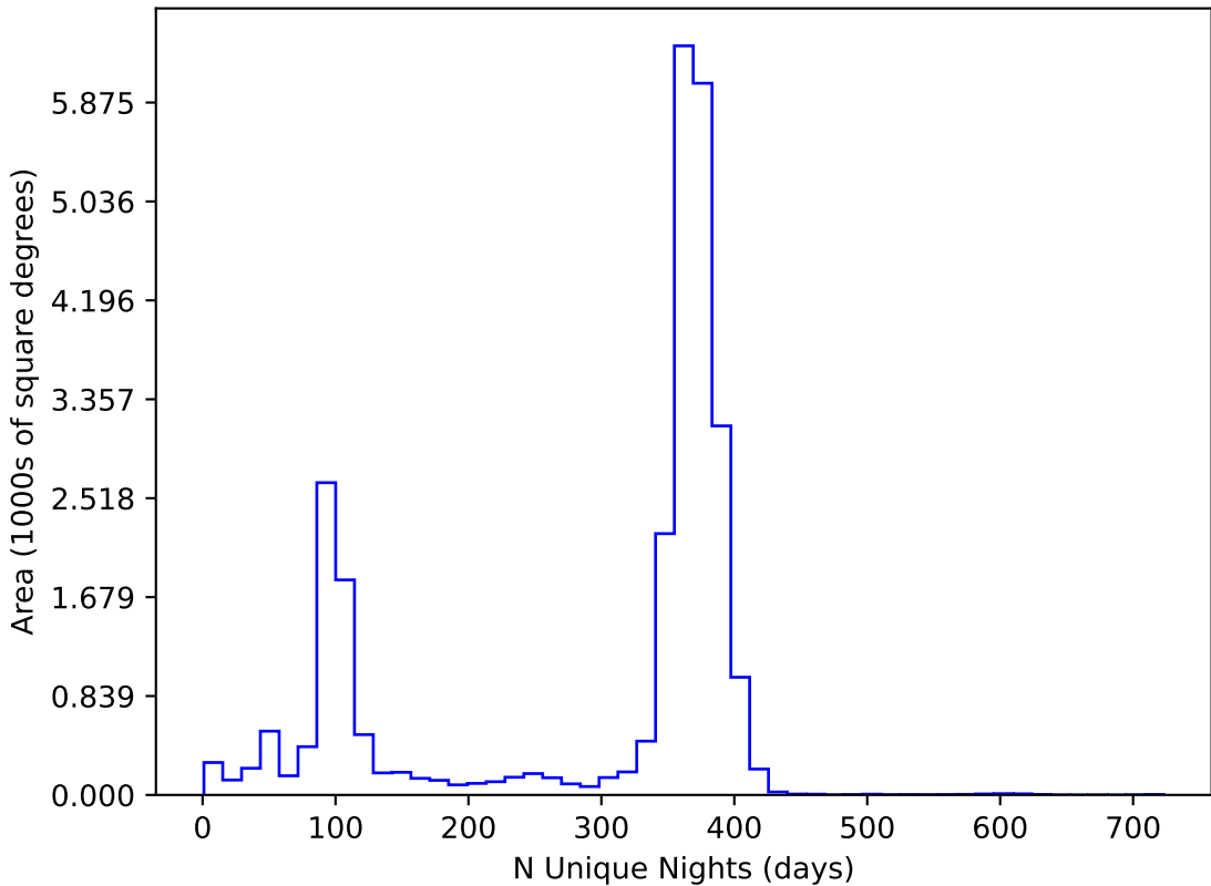
roll_pause_mjdp270_v3.4_10yrs All sky all bands: N Unique Nights
