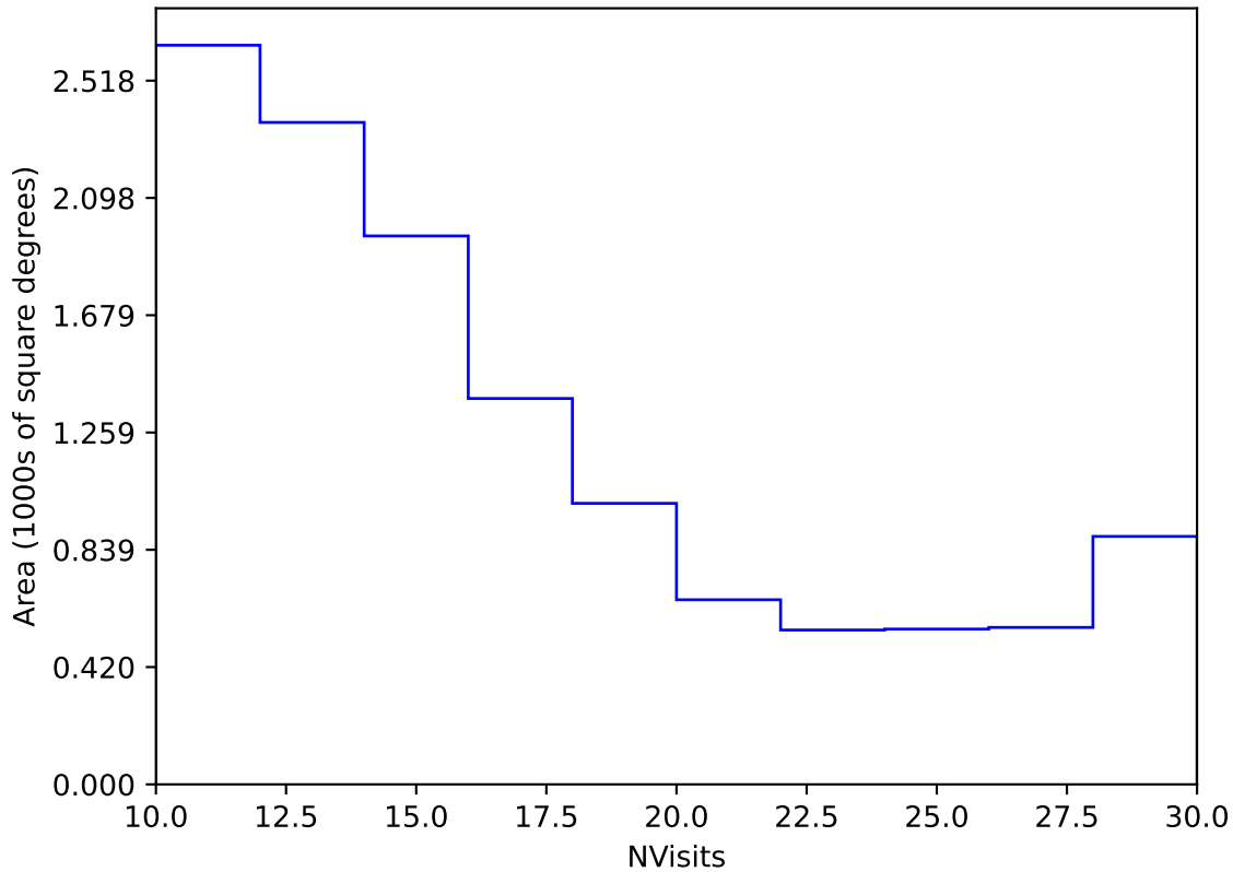
roll_pause_mjdp270_v3.4_10yrs Yr 3-4 y band: NVisits
