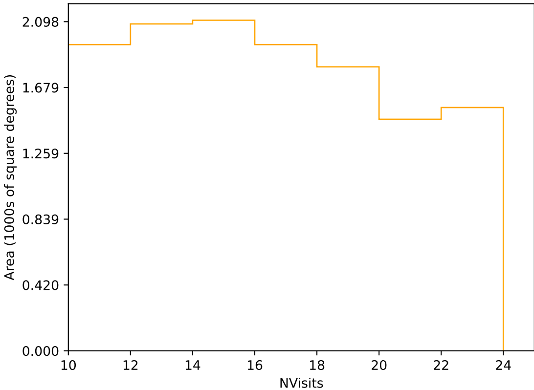
roll_pause_mjdp270_v3.4_10yrs Yr 3-4 r band: NVisits
