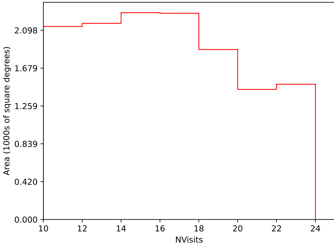
roll_pause_mjdp270_v3.4_10yrs Yr 3-4 i band: NVisits
