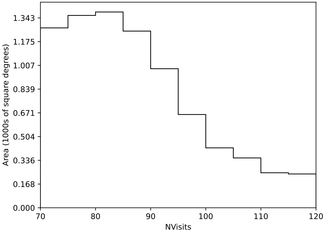
roll_pause_mjdp270_v3.4_10yrs Yr 3-4 all bands: NVisits
