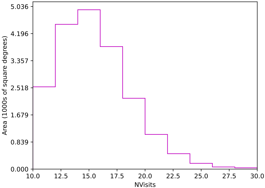
roll_pause_mjdp270_v3.4_10yrs Yr 1 z band: NVisits
